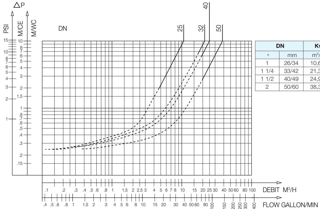
PULSAIR 3 - Headloss chart
