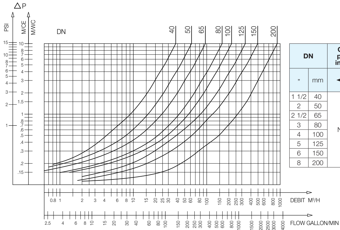
407 - Headloss chart
